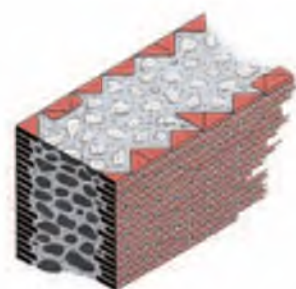
V. Opus testaceum
